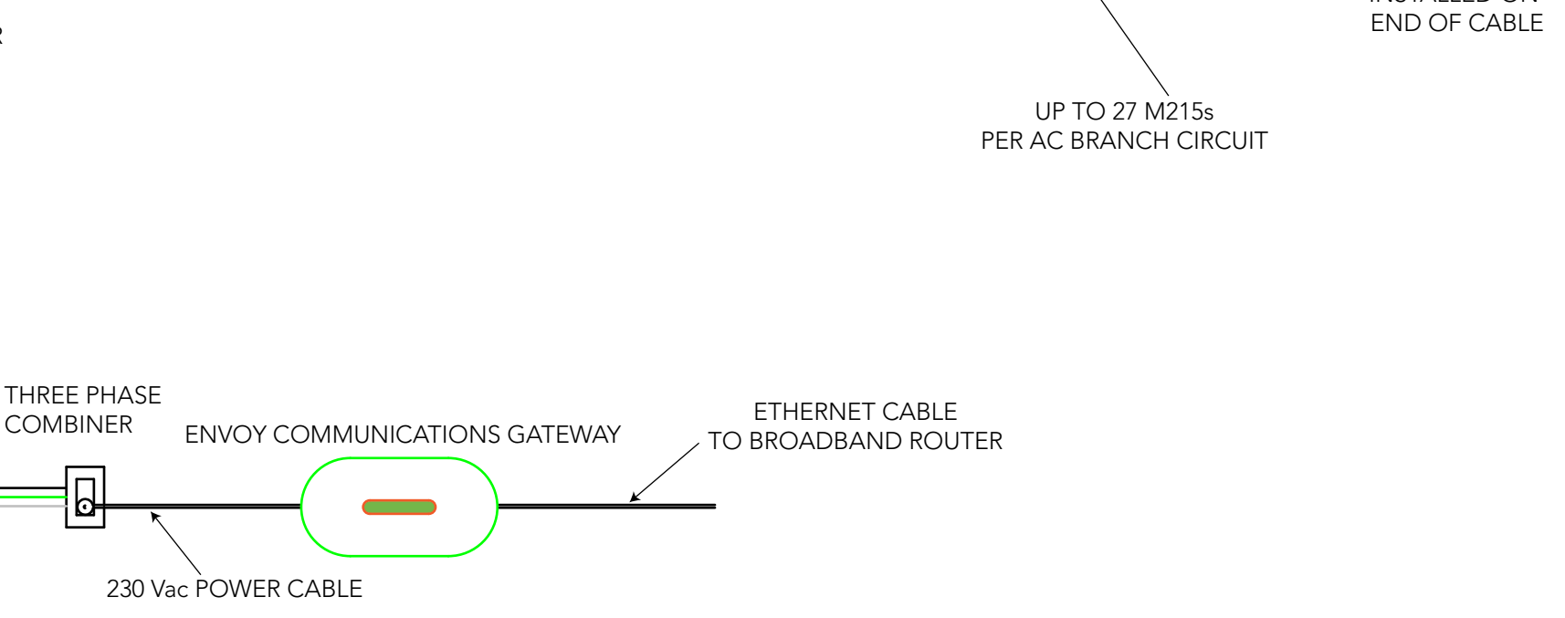
FIELD WIRING DIAGRAM THREE PHASE
